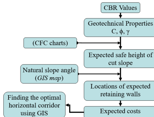
Figure (10): Flowchart of using retaining wall costs in extracting the horizontal road corridor using GIS
