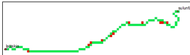
Figure (9): Deviation of the horizontal corridor due to retaining wall requirements in the cut area
