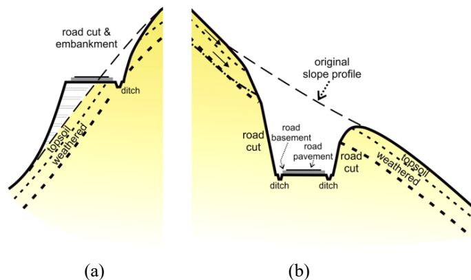
Figures (4): Roadside retaining walls in a mountainous terrain: (a) road cut and embankment; (b) road cuts
