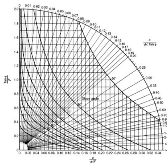
Figure (5): Circular failure chart according to Hoek and Bray (1981)
